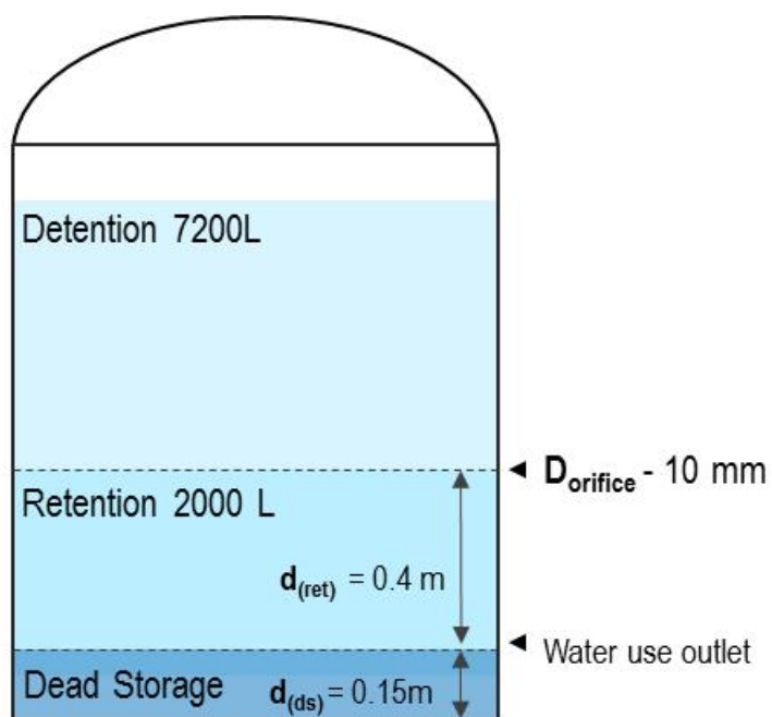
Figure 41: Rainwater tank specifications for mitigation of 500 m 2 roof (10000 L)
