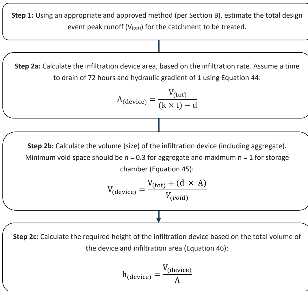
Figure 46: Infiltration design flow chart
