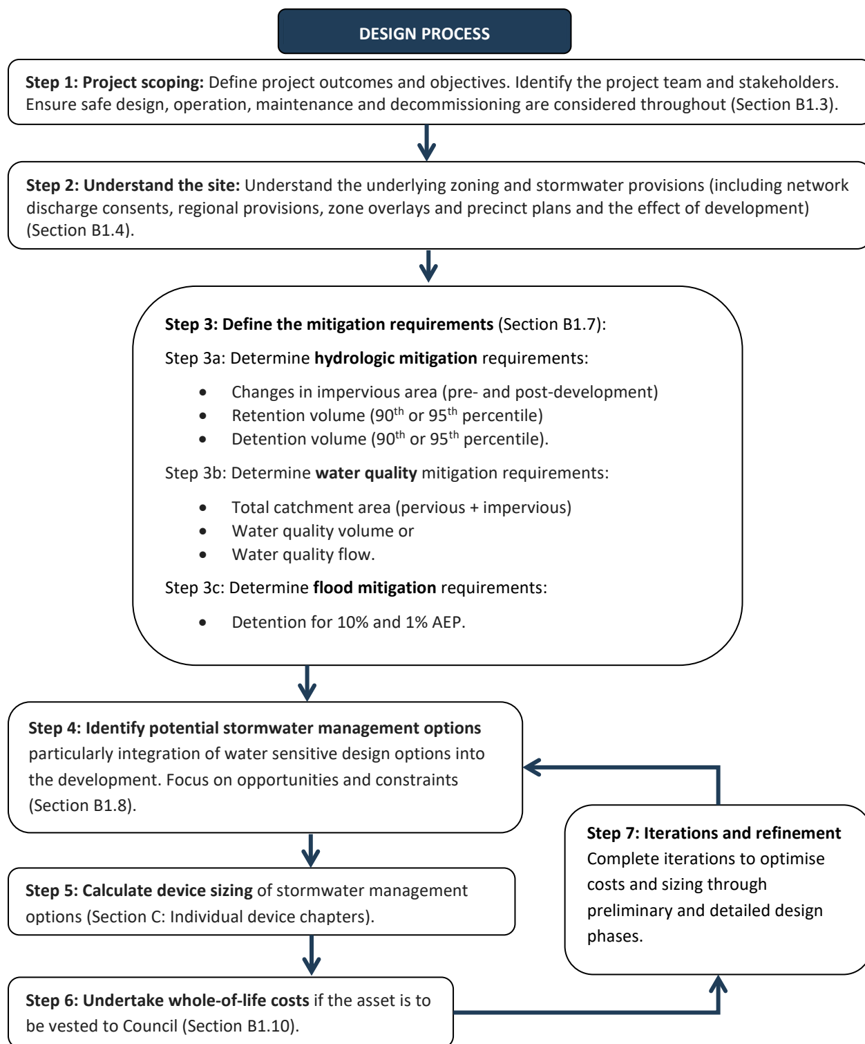
Figure 4: Recommended design process for stormwater management
