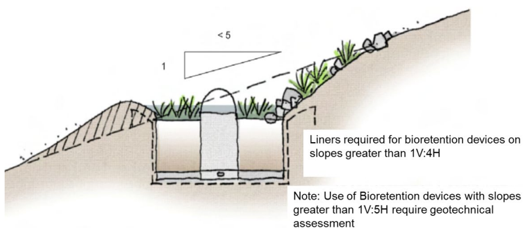
Figure 22: Schematic of slope constraints and liner use
