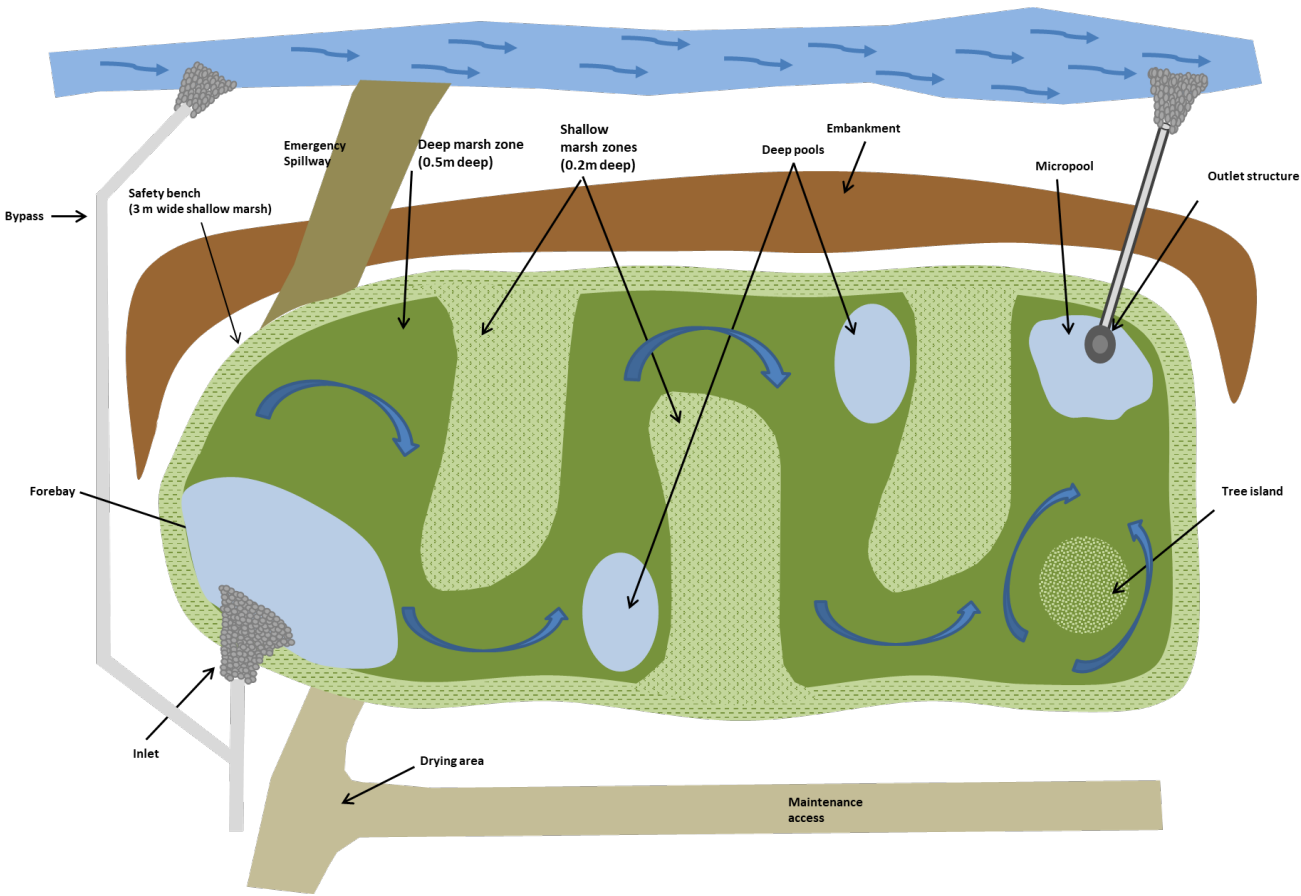
Figure 51: Example schematic of a sinuous bathymetry wetland
