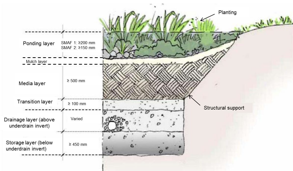
Figure 15: Schematic of rain garden cross-section
