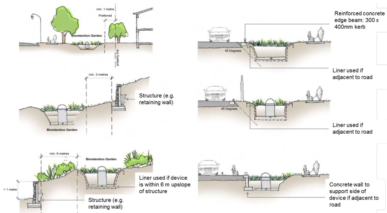
Figure 21: Setback limitations for bioretention devices
