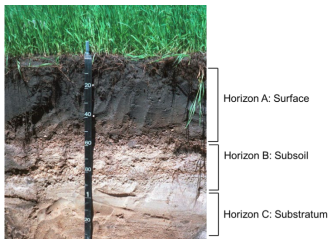
Figure 8: Soil profile example
