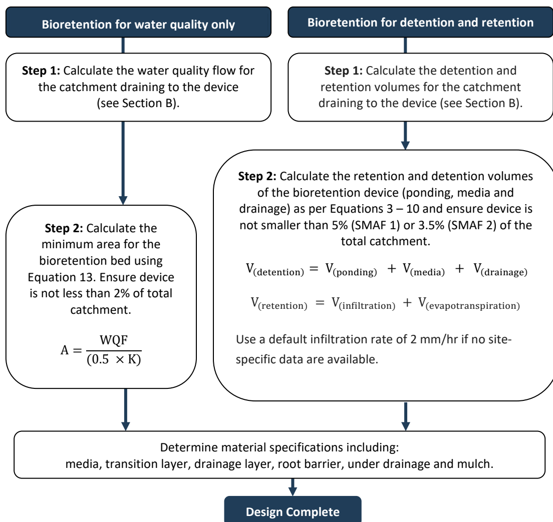
Figure 24: Bioretention device design flow chart
